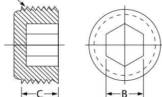
Dimension NPT
